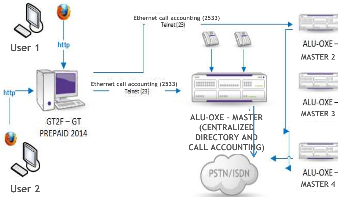
Standalone call accounting directories setup: multi-sites (1 link by master)
