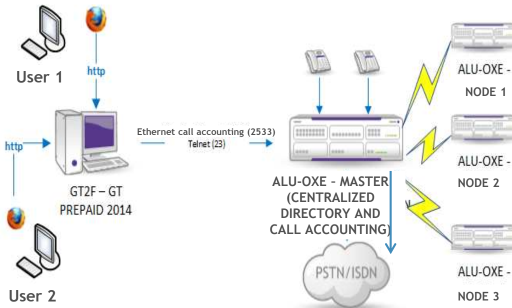
Standalone call accounting directories setup: multi-sites (1 link by master)
